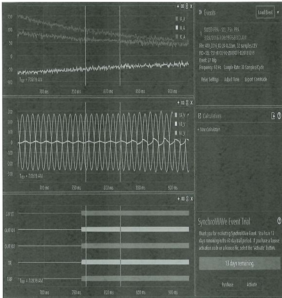
Figure 5: Single-Phase Power Quality Event
