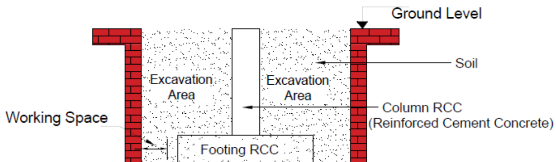
Footing Details
