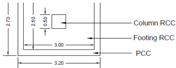
Footing Details
